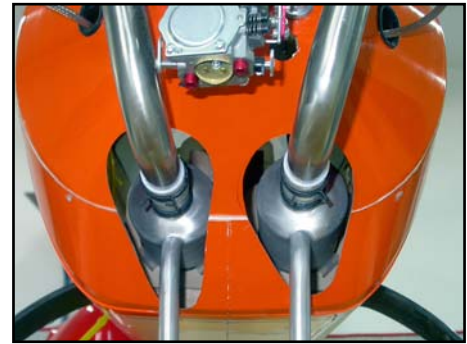
(above) Cut large enough holes to insert the cans through the motordome, taking note of the cooling requirements mentioned here.
