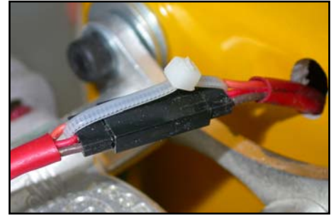
(below) Secure the connectors between the motor & ignition unit. (below) Fit barbs to all brass tubes and fuel connections for safety. Easily made from a paper-clip, soldered onto the brass tubes.
