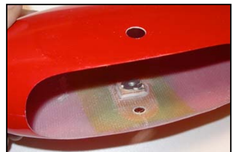
(above & below) Glue the milled plywood reinforcements to the inside & outside of the wheelpant as shown. The inside plate will have an M3 T-nut glued to it later.
