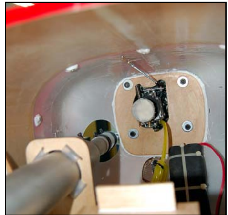
(below) Standoffs are bolted thru' the firewall with the supplied M6 x 20mm allen bolts & washers. M6 T-nuts are also included in the hardware, which can be used with some engine mount types.
