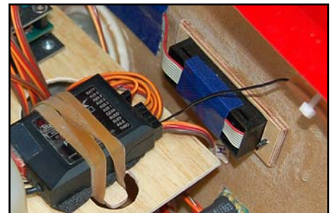
(above) 3mm plywood reinforcing plate glued inside the cutouts in the fuselage sides for switches.
