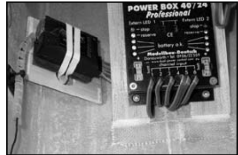
(above) The Powerbox can be screwed to the plate behind the rudder servos if using a DA-100.
