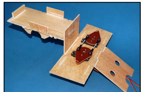
(below) The Tank base/Rudder tray is assembled from the milled parts included in the kit.
